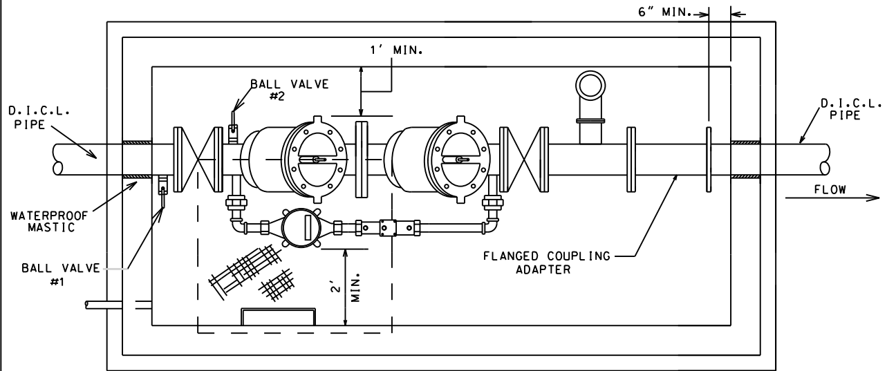
SECTIONAL PLAN
