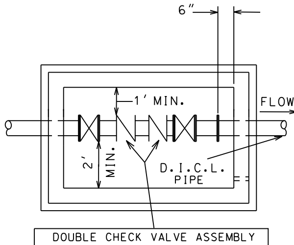
SECTIONAL PLAN
