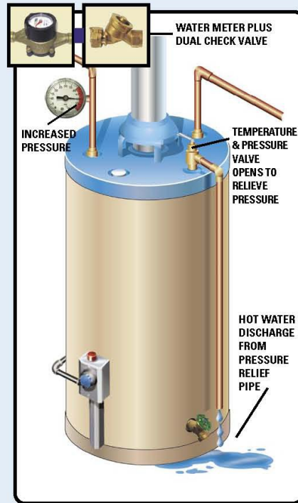
DUAL CHECK VALVE INSTALLED AT METER
